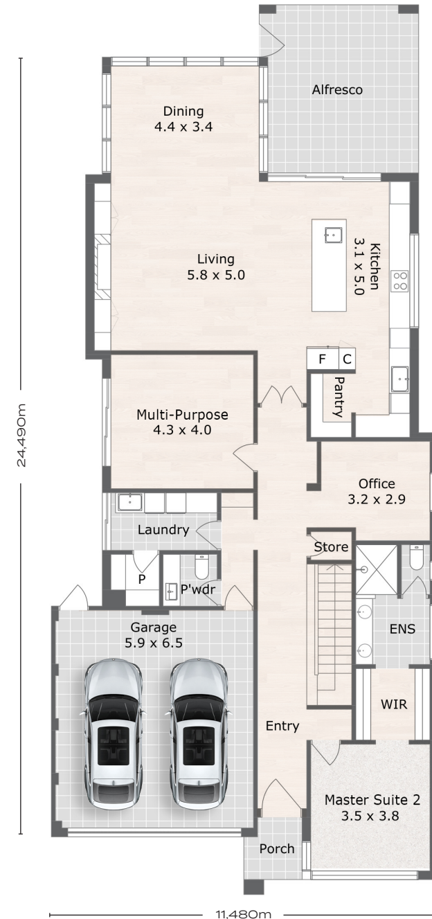
GROUND FLOOR
